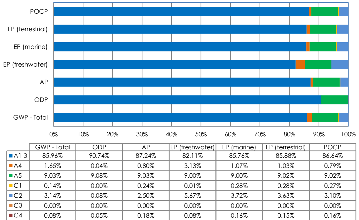
Figure 1 - shows the relative contribution of each life cycle stage to different environmental indicators for the carbon steel reinforcing bar products manufactured by the primary (DRI) and the secondary (scrap-based) production routes
